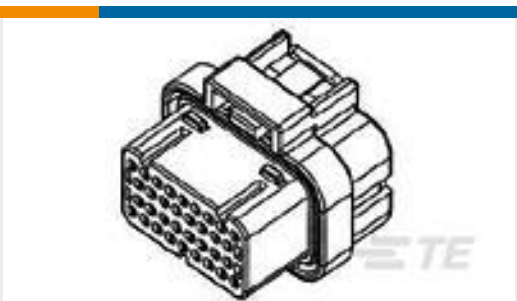
TE Part #4-1437290-0 34POS,SUPERSEAL,REC HSG ASSY, SLD,COD 1
