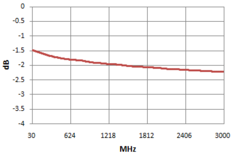
Insertion Loss
