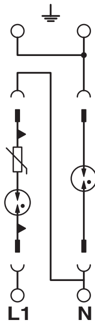
Circuit diagram
