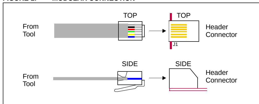
FIGURE 1: MODULAR CONNECTION
