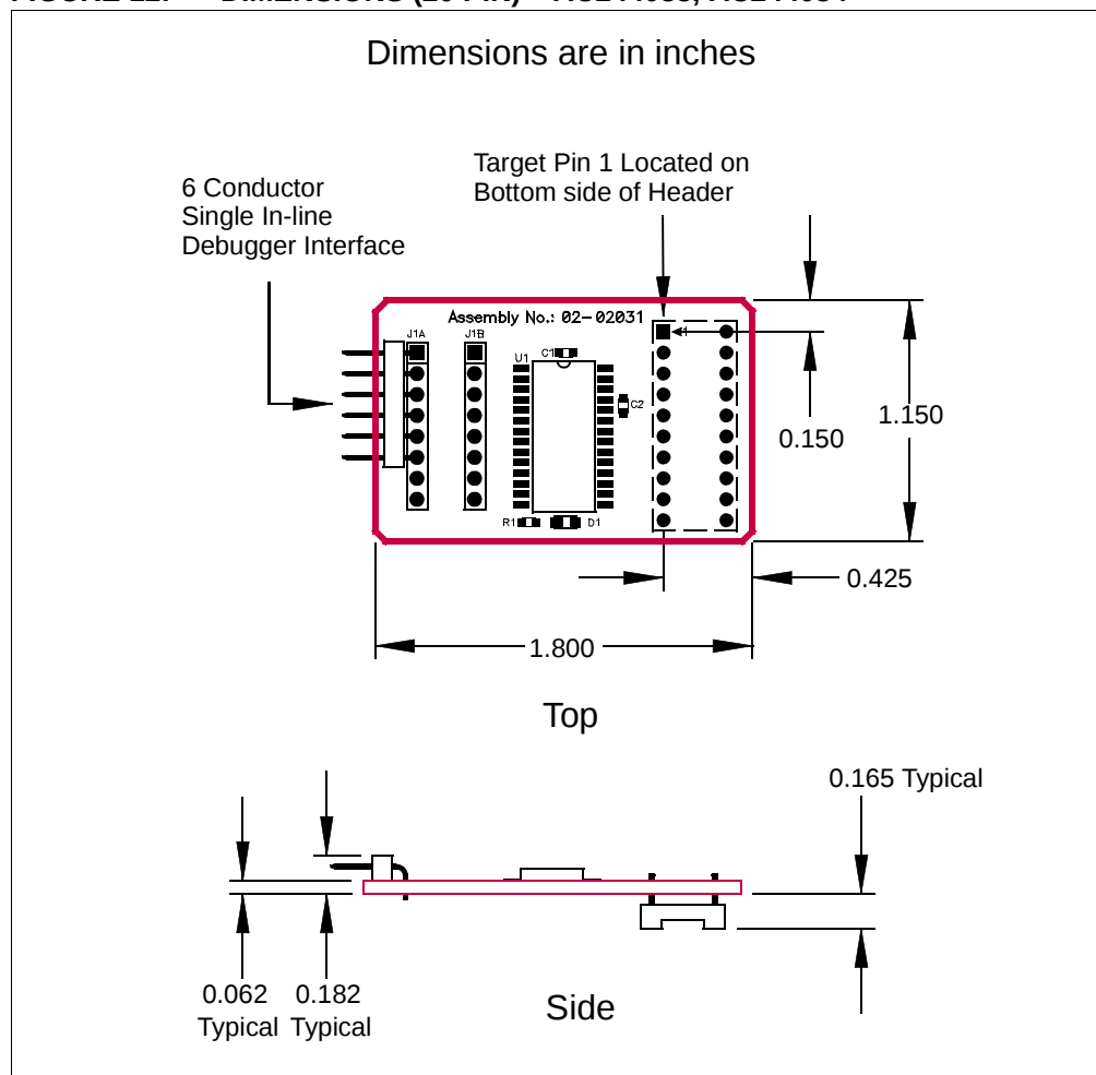
FIGURE 12: DIMENSIONS (20 PIN) – AC244033, AC244034
