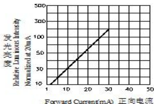
正向电流 Fig.4 Relative Luminous Intensity vs Forward Current
