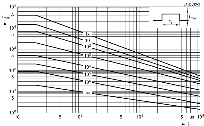
SIOV-B40K550 ... K750
