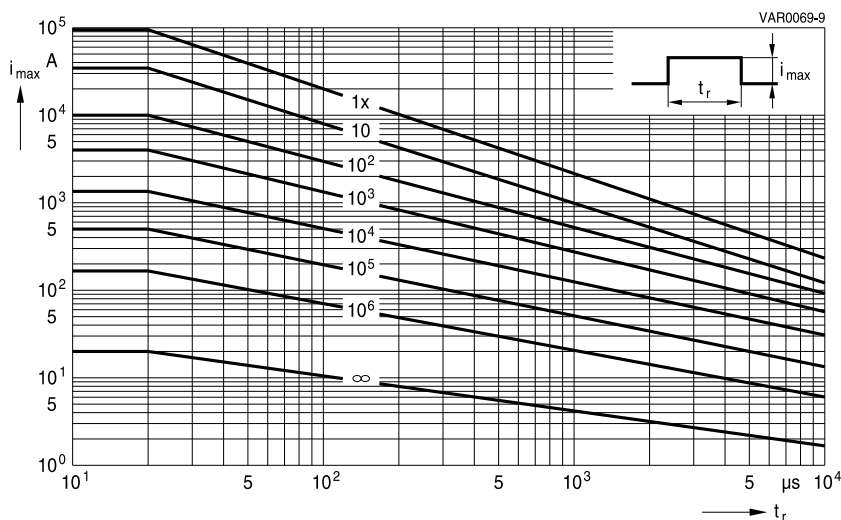
SIOV-B80K130 ... K1100
