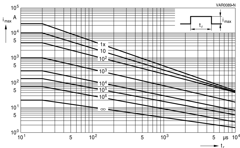
SIOV-B32K230 ... K460
