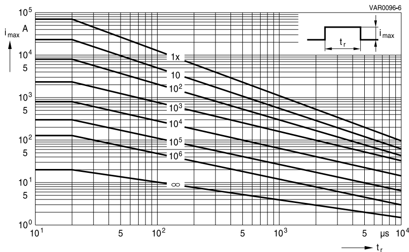
SIOV-B60K550 ... K1000
