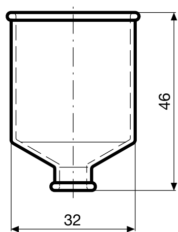
Accessories TZZ06 Protective cover rear side IP41
