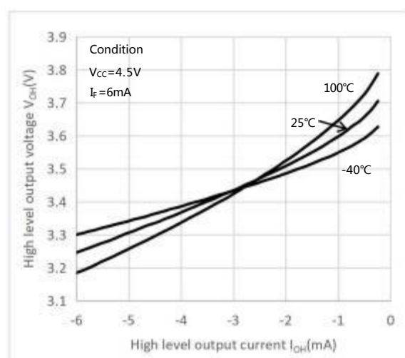
Fig.8 High level output voltage vs. High output current
