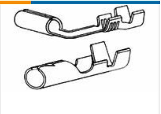
TE Part #42700-1 SHUR PLUG 180 RECEPTACLE 20-16 AWG BR
