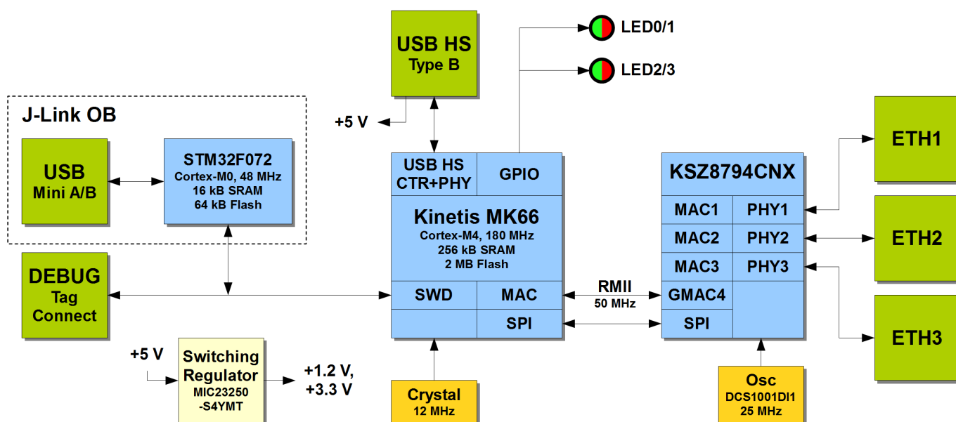
embOS/IP Switch Board V2 Block Diagram
