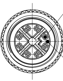
M12 X-CODE MALE FRONT VIEW
