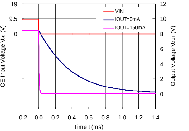
R1517J251F (C2 = 0.1 μF, CD = 1 nF)
