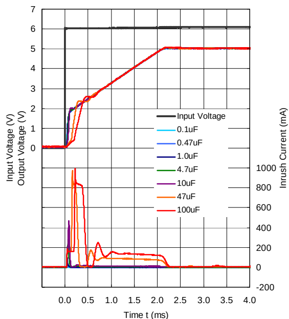
R1517J501E/F ( C_D = 10 \text{ nF} )
