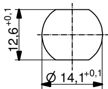
Cut-Out Front Panel
