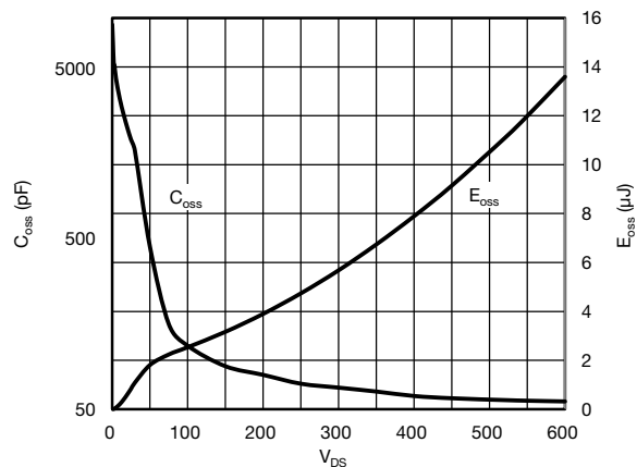
Fig. 5 - Typical Capacitance vs. Drain-to-Source Voltage
