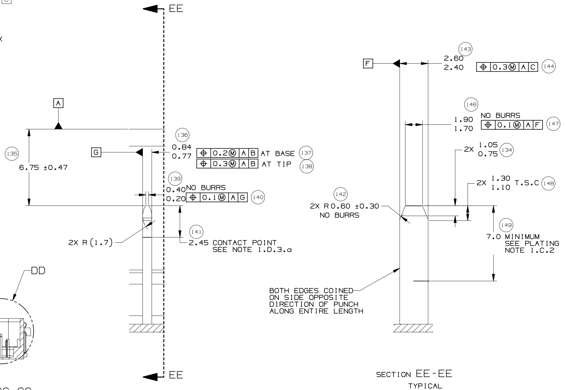
DETAIL DD TYPICAL SCALE 5:1
