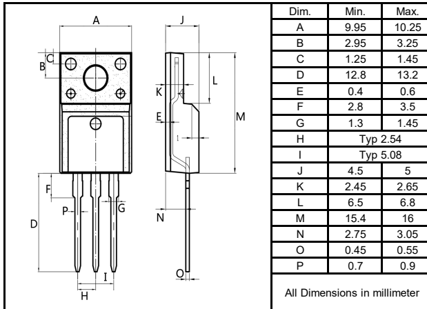
T0-220F
