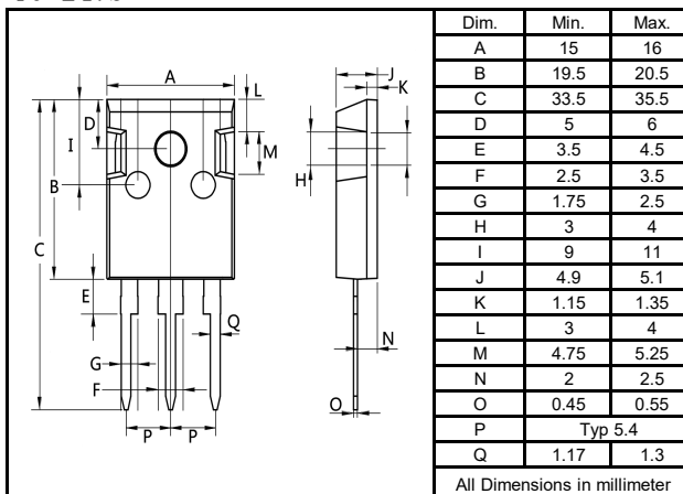
T0-247S
