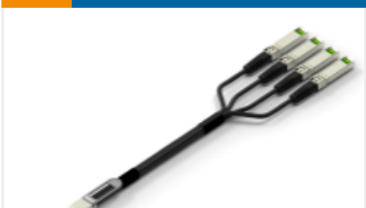
TE Part #4-2334236-4 QSFP56-Four SFP56 Cable Assembly: 30 AWG
