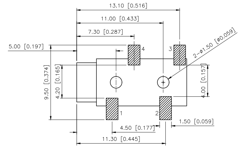
P.C.B LAYOUT MOUNTING PATTERN (TOP VIEW)
