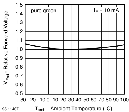
Figure 26. Relative Forward Voltage vs. Ambient Temperature
