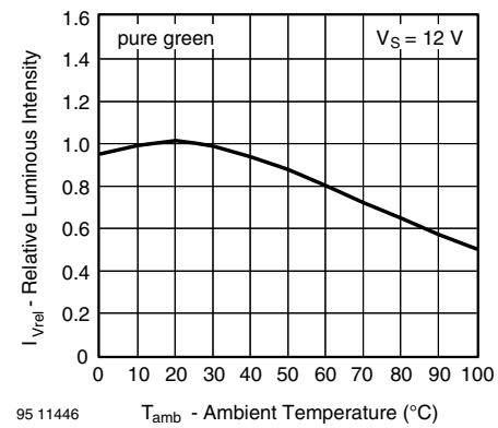
Figure 28. Rel. Luminous Intensity vs. Ambient Temperature
