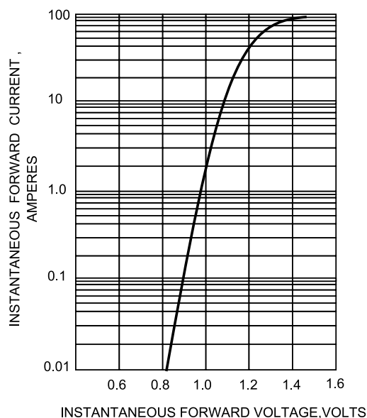
FIG.3-TYPICAL FORWARD CHARACTERISTICS
