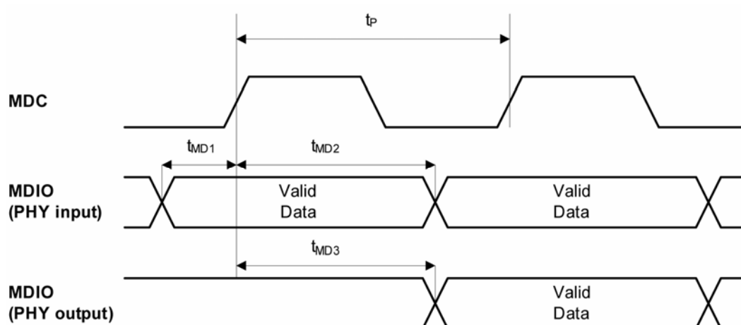
Figure 17. MDC/MDIO Timing
