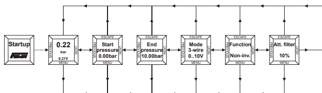
Fig. 4. Menu structure (excerpt)
