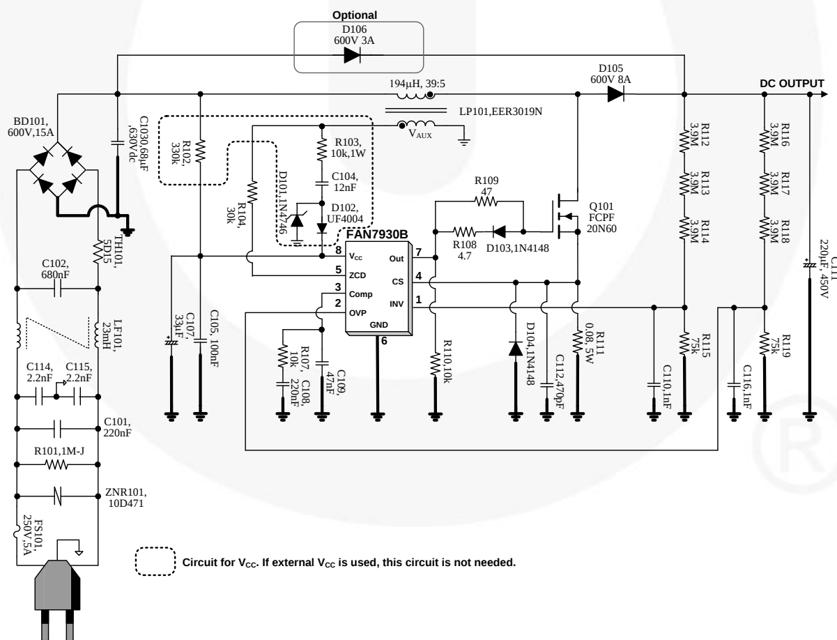
Figure 44. Demonstration Circuit
