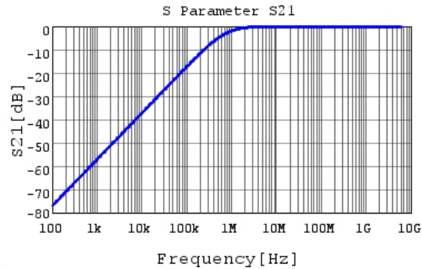
GRM15XB11E222KA86 S21 DC0V,20degC
