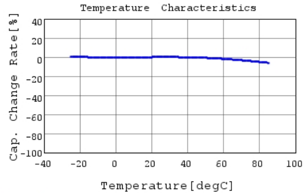
GRM15XB11E222KA86 C-Temp. capchange, DC0.0V,
