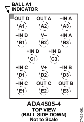
Figure 6. 14-Ball WLCSP (CB-14-1)
