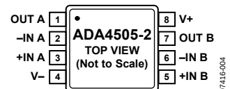
Figure 2. 8-Lead MSOP (RM-8)
