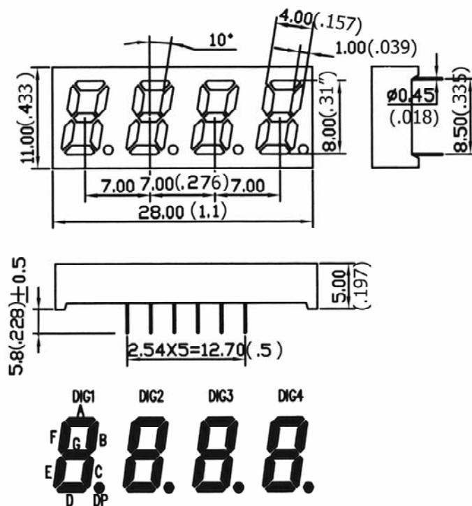
KW4-311AGA
