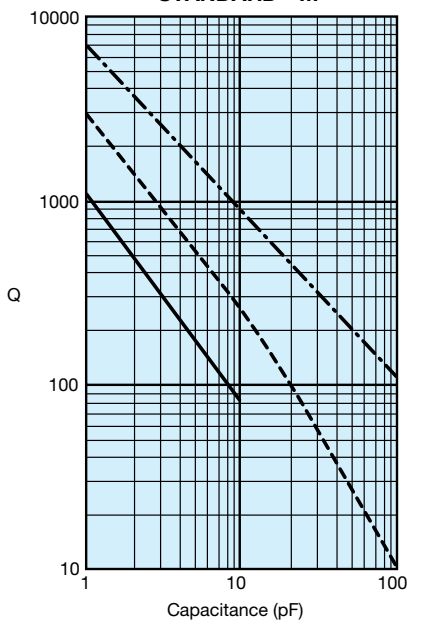
TYPICAL Q vs. CAPACITANCE AQ13/14 MIL-PRF-55681E - BG STANDARD - M
