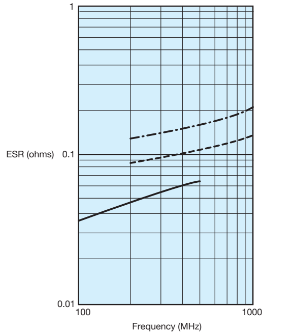
TYPICAL ESR vs. FREQUENCY AQ13/14 MIL-PRF-55681E - BP STANDARD - A
