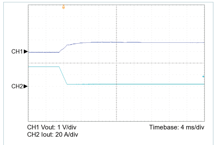
Figure 7 — 100% to 10% load transient response, V_{IN} = 270\text{ V} , nominal trim, C_{OUT\_EXT} = 680\text{ }\mu\text{F}
