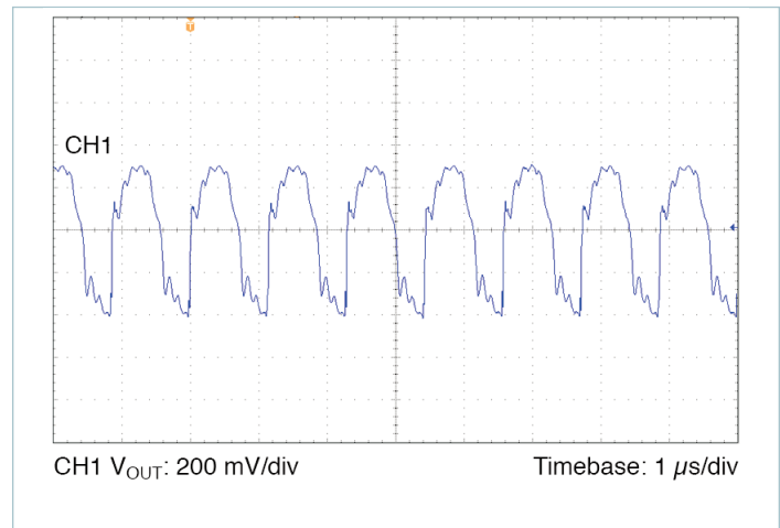
Figure 19 — Output voltage ripple, V_{IN} = 270\text{ V} , V_{OUT} = 15.0\text{ V} , C_{OUT\_EXT} = 680\text{ }\mu\text{F} , R_{LOAD} = 0.449\text{ }\Omega
