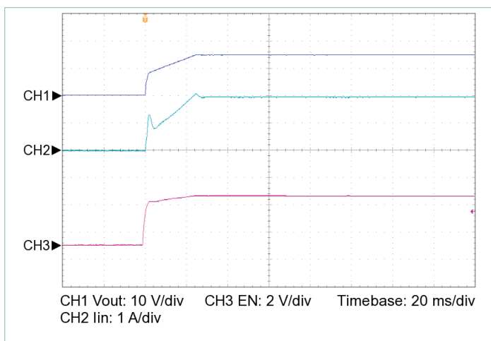
Figure 17 — Startup from EN, V_{IN} = 270\text{ V} , C_{OUT\_EXT} = 6800\text{ }\mu\text{F} , R_{LOAD} = 0.449\text{ }\Omega
