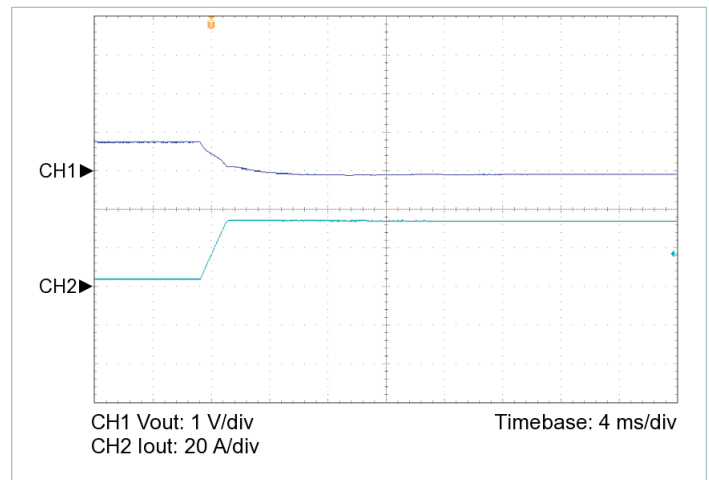
Figure 8 — 10% to 100% load transient response, V_{IN} = 270\text{ V} , nominal trim, C_{OUT\_EXT} = 680\text{ }\mu\text{F}
