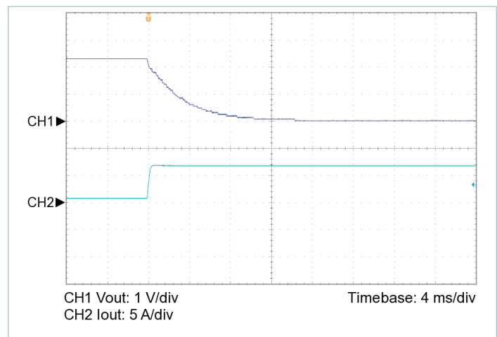
Figure 8 — 10% to 100% load transient response, V_{IN} = 28\text{ V} , nominal trim, C_{OUT\_EXT} = 200\text{ }\mu\text{F}
