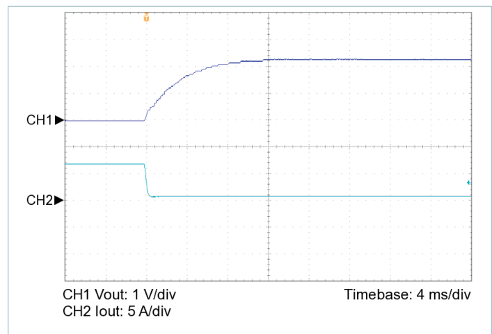
Figure 7 — 100% to 10% load transient response, V_{IN} = 28\text{ V} , nominal trim, C_{OUT\_EXT} = 200\text{ }\mu\text{F}
