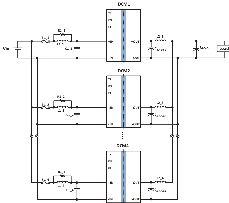
Typical Application 1: DCM3623x75X1380yzz in an array of four units
