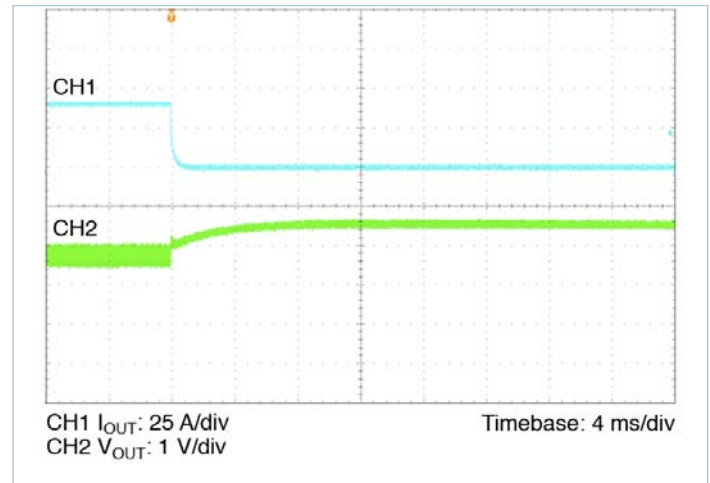
Figure 19 — 100% to 10% load transient response, V_{IN} = 290\text{V} , nominal trim, C_{OUT\_EXT} = 1000\mu\text{F}
