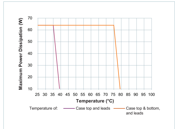
Figure 27 — Maximum Power Dissipation for Array or Current Limit Operation
