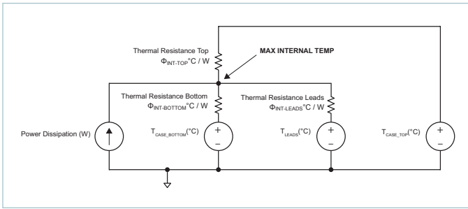
Figure 22 — Double side cooling and leads thermal model
