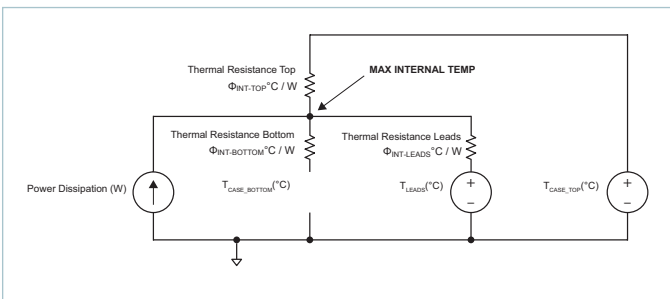
Figure 23 — One side cooling and leads thermal model
