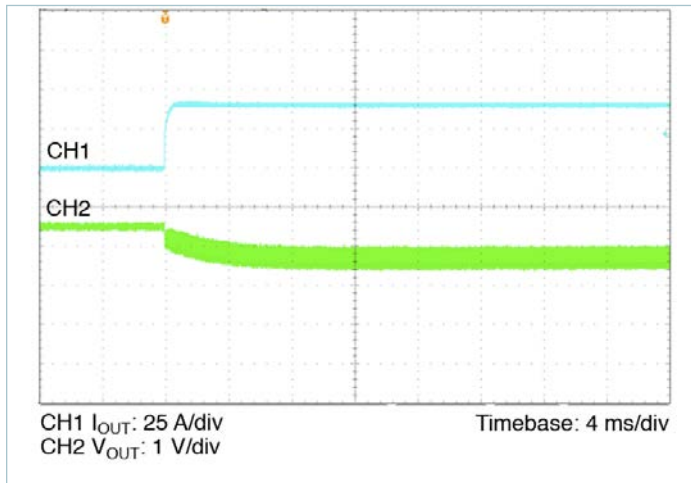
Figure 16 — 10% to 100% load transient response, V_{IN} = 290\text{V} , nominal trim, C_{OUT\_EXT} = 1000\mu\text{F}
