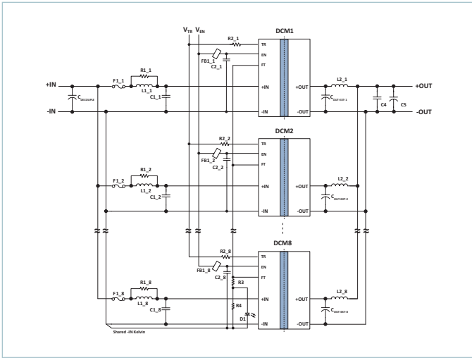
Figure 25 — DCM paralleling configuration circuit 1
