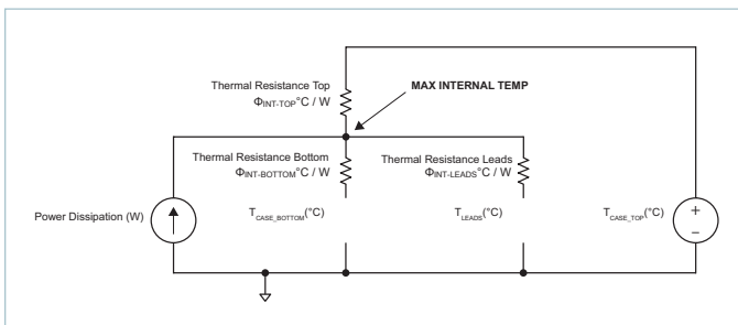
Figure 24 — One side cooling thermal model
