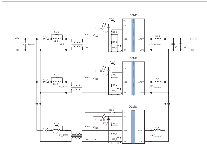
Figure 26 — DCM paralleling configuration circuit 2
