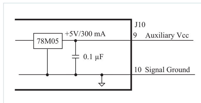
Figure 7. Auxiliary Vcc
