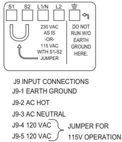
Input Panel Connectors
