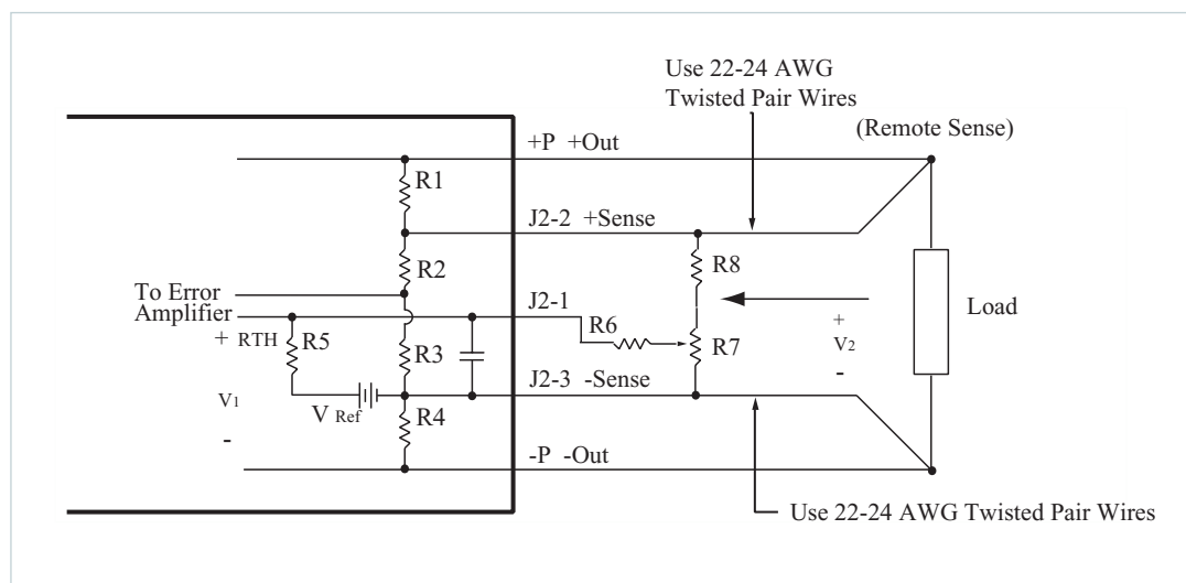
Figure 10. External Trim
