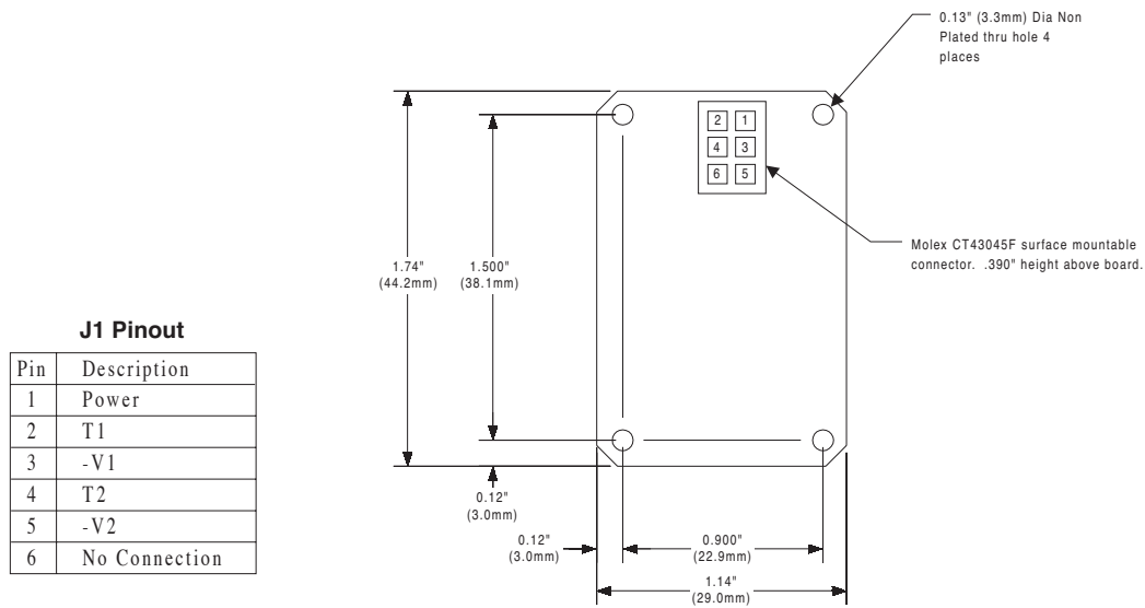
Figure 12. Mechanical Drawing
