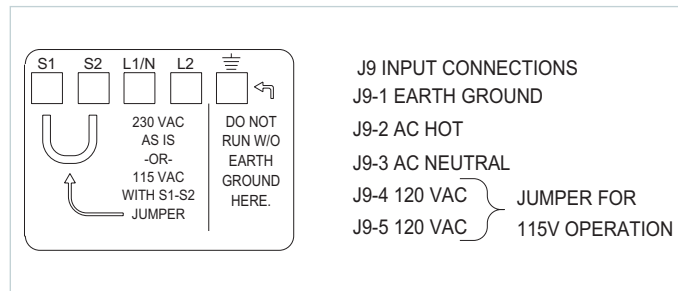
Figure 3. Input Panel Connectors
