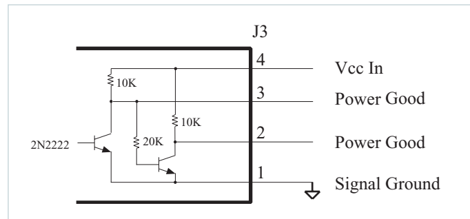
Figure 8. Power Good and Vcc
