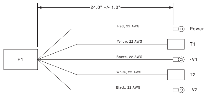
Figure 13. Cable Drawing
