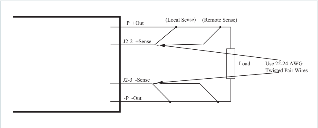
Figure 9. Sense Leads
