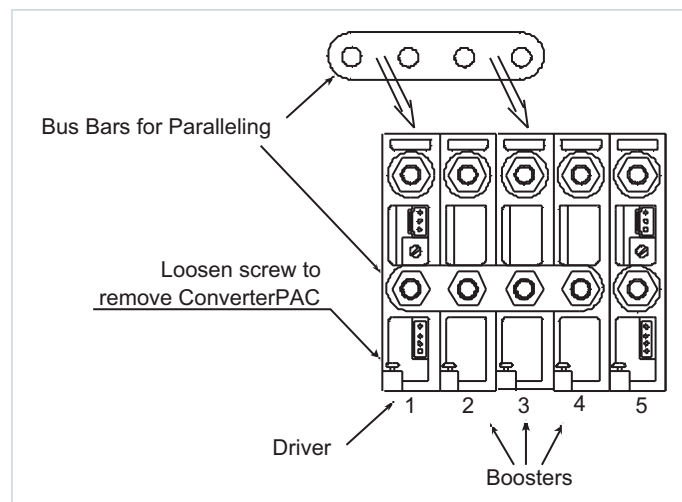
Figure 2. Paralleling ConverterPACs
