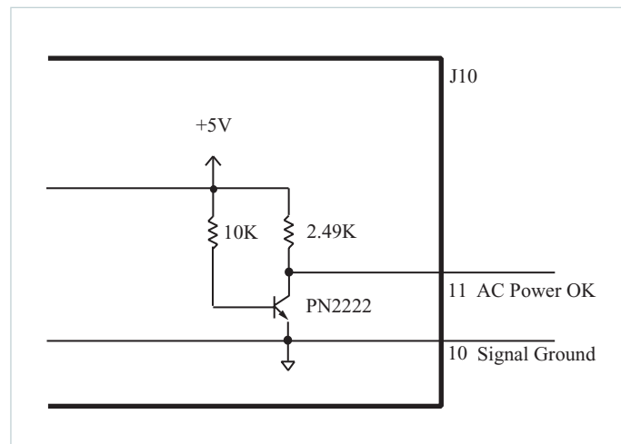
Figure 6. AC OK / Power Fail
