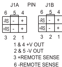
DualPAC Output Connector
