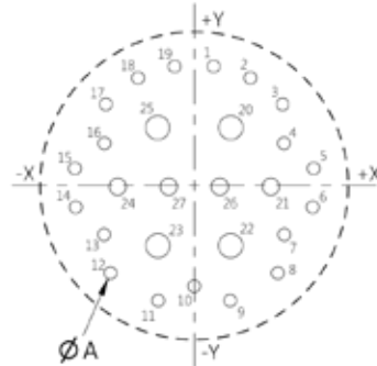
19 Contacts Size 20 4 Contacts Size 16 4 Contacts Size 12
