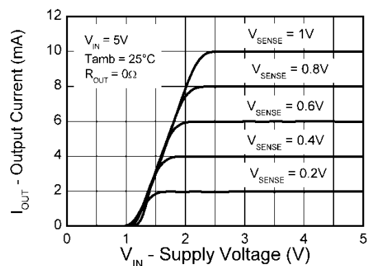
Transfer Characteristic
