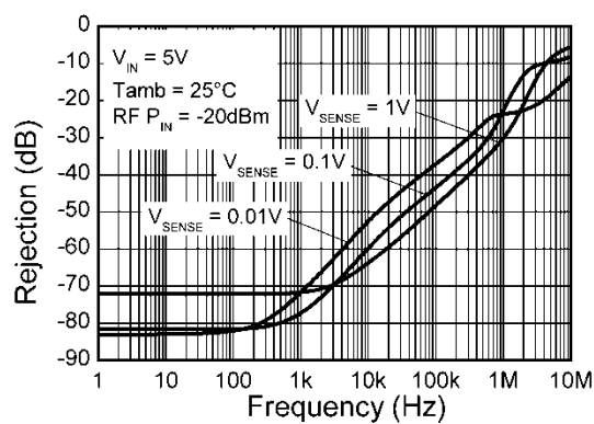
Common Mode Rejection
