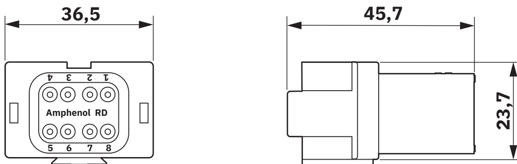
AT04-08PA top view and side view
