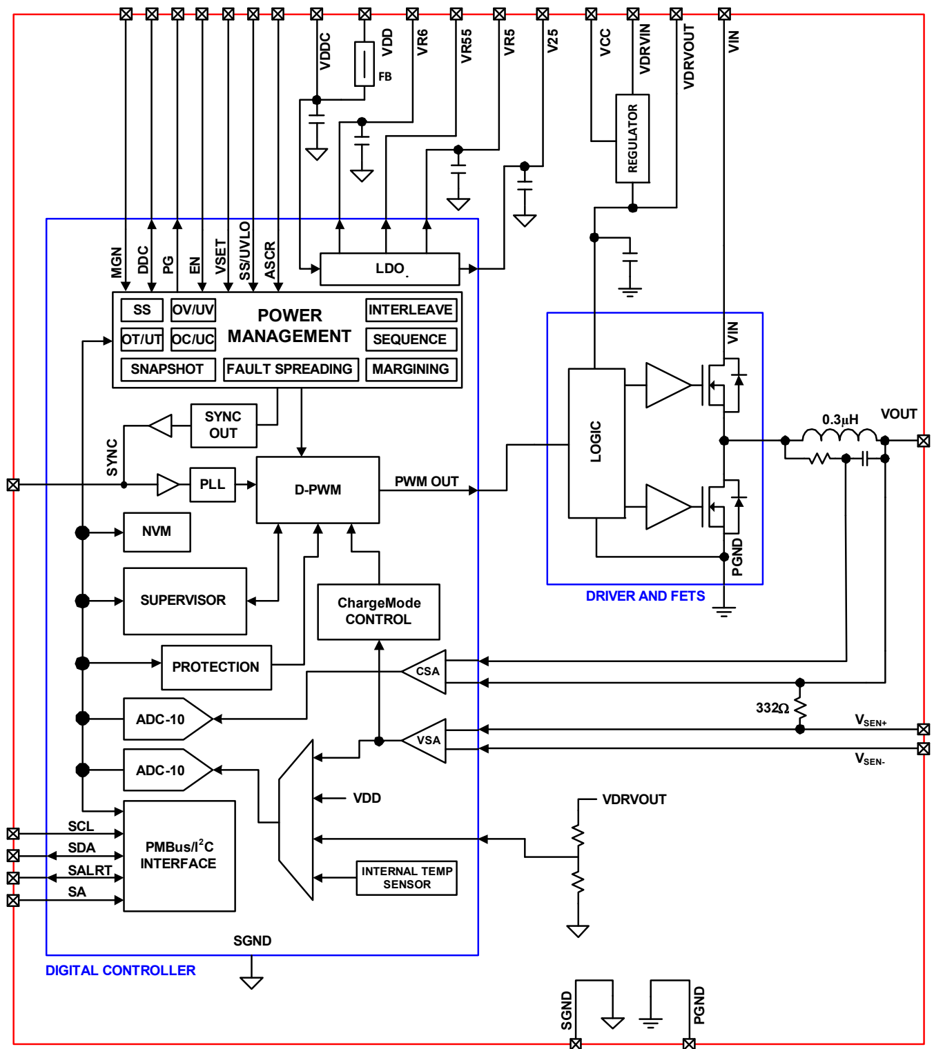
FIGURE 3. BLOCK DIAGRAM
