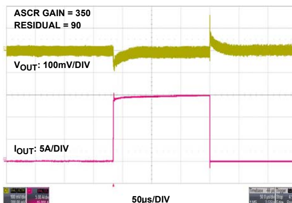
FIGURE 15. 12V IN TO 5V OUT TRANSIENT RESPONSE, f_{SW} = 727kHz , C_{OUT} = 3 \times 100\mu F CERAMIC + 2 \times 470\mu F POSCAP
