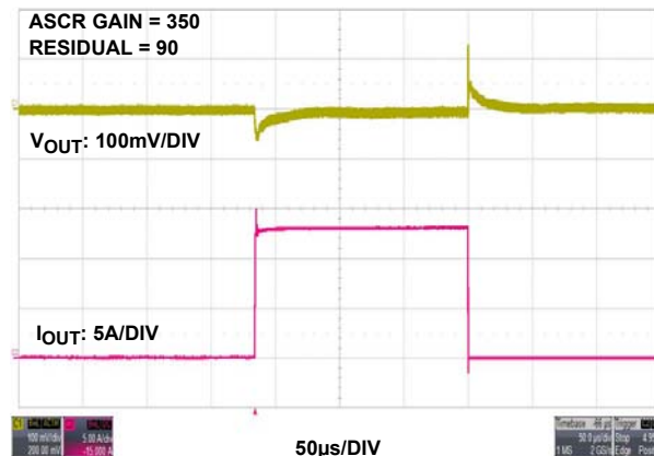
FIGURE 11. 5V IN TO 1.8V OUT TRANSIENT RESPONSE, f_{SW} = 615kHz , C_{OUT} = 3 \times 100\mu F CERAMIC + 2 \times 470\mu F POSCAP
