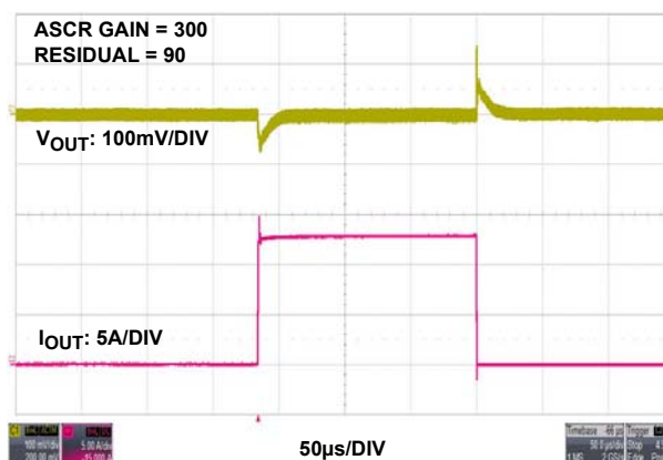
FIGURE 13. 12V IN TO 1.8V OUT TRANSIENT RESPONSE, f_{SW} = 615kHz , C_{OUT} = 3 \times 100\mu F CERAMIC + 2 \times 470\mu F POSCAP
