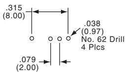
PCB Hole Layout
