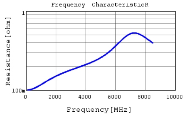
GJM1555C1H5R4BB01 R DCOV, 25degC
