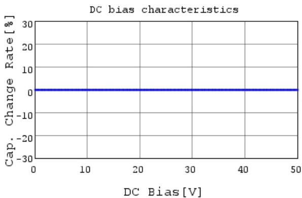
GJM1555C1H5R4BB01 C-DC bias capchange, 25.0C
