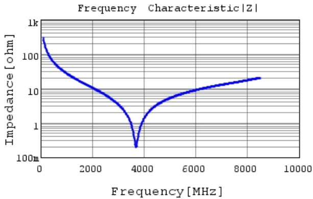
GJM1555C1H5R4BB01 |Z| DCOV, 25degC
