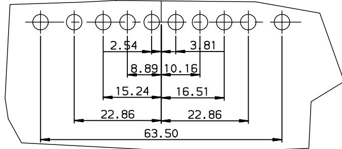
LAYOUT DIMENSIONS (after plating) CONNECTOR SIDE VIEW
