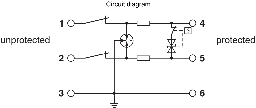
Schematic diagram
