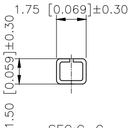
SEC:C-C
