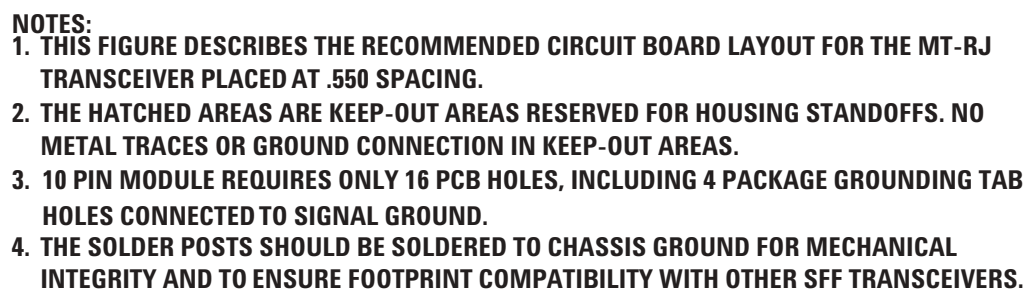
Figure 9. Recommended Board Layout Hole Pattern
