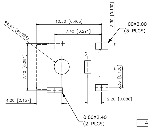
PCB LAYOUT
