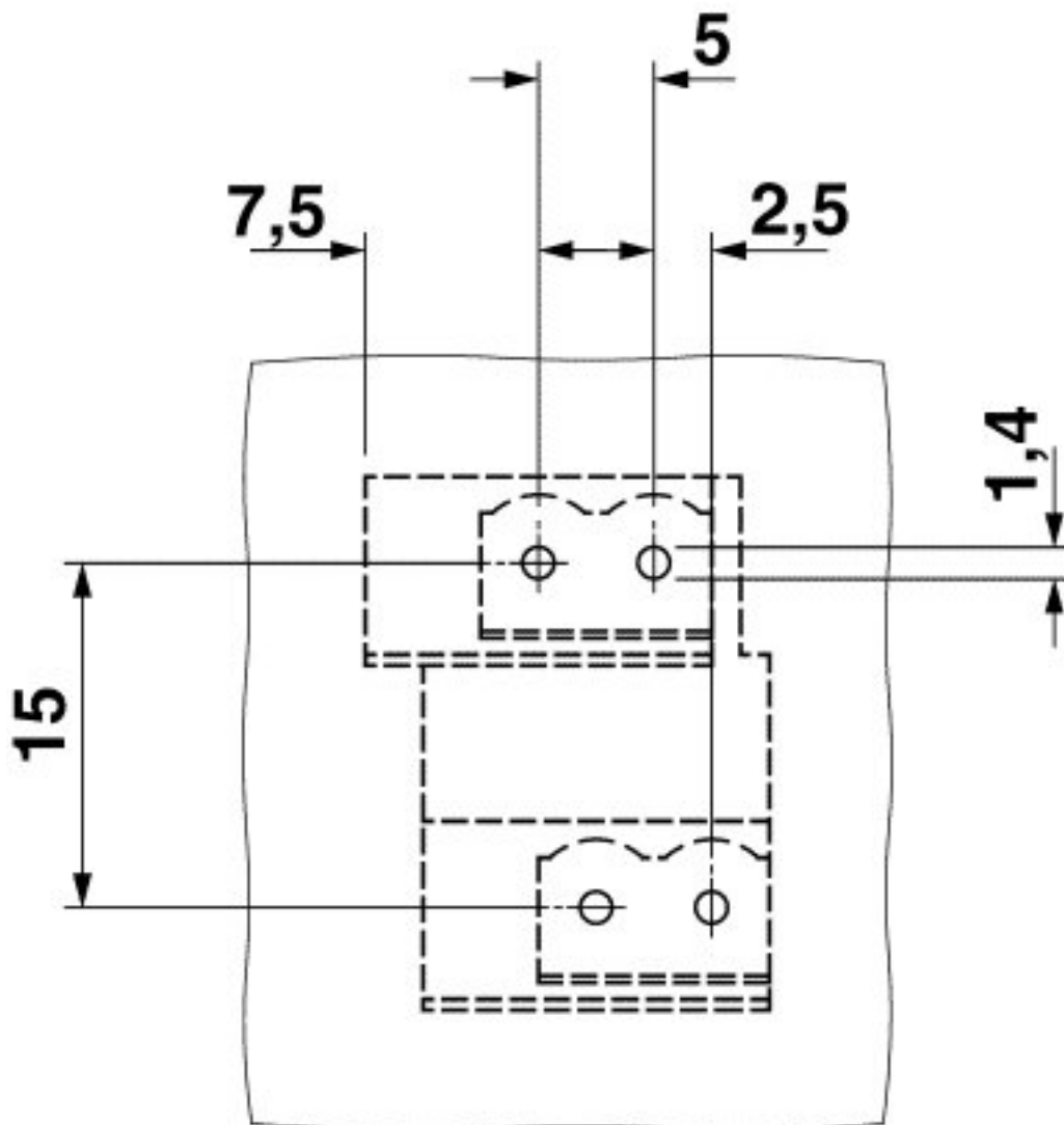
Drilling diagram
