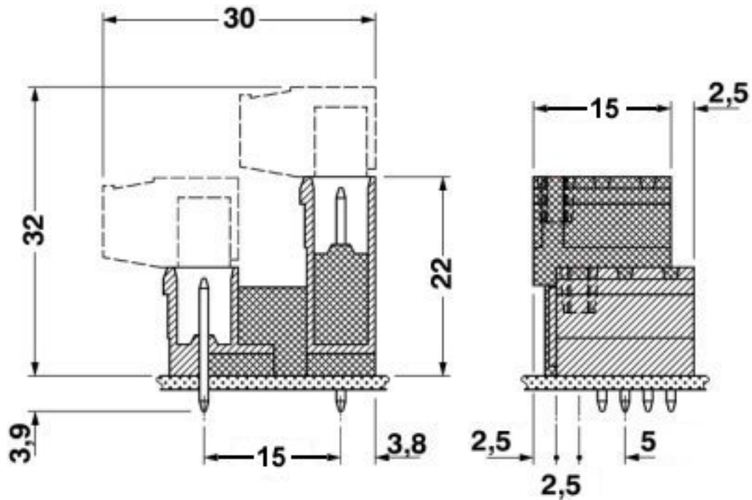
Dimensioned drawing
