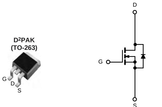
N-Channel MOSFET
