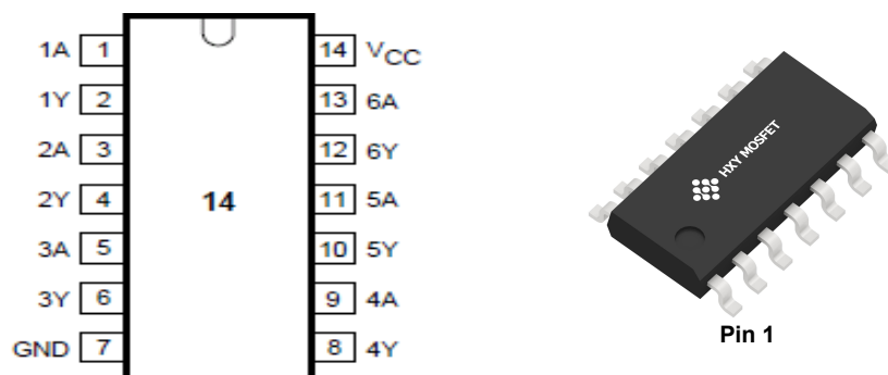
Fig.3 Pin configuration
