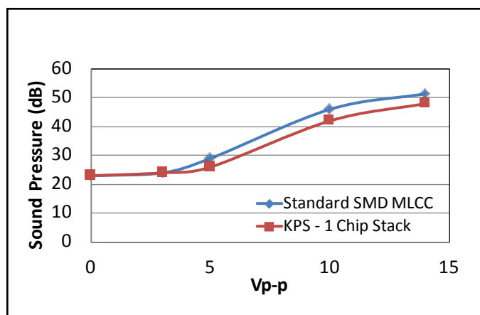
Microphonics – 1210, 4.7 \mu F, 50 V, X7R
