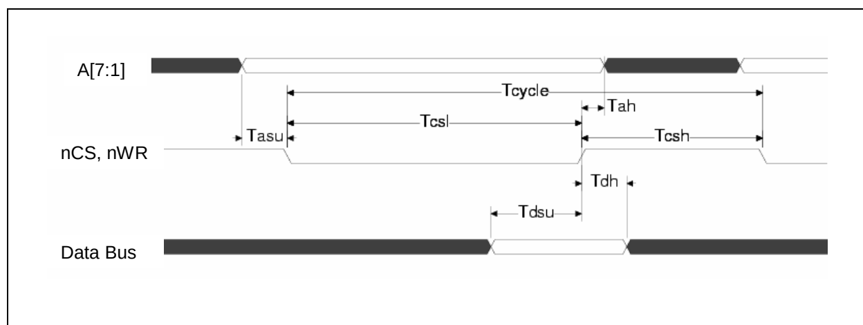
Figure 6.5 PIO Write Cycle Timing
