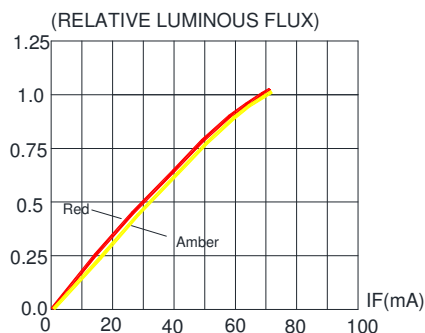
FIG.2 RELATIVE LUMINOUS FLUX VS. FORWARD CURRENT
