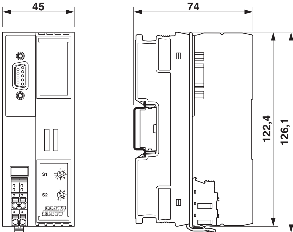
Dimensional drawing
